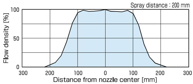
Flow distribution along long side
