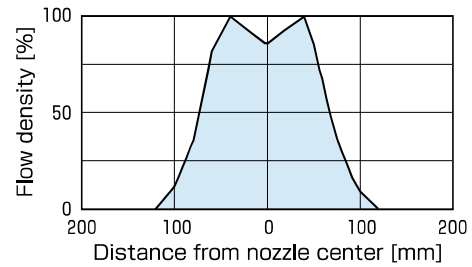
Flow distribution along short side
